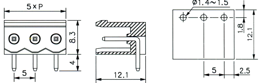
PCB LAYOUT
